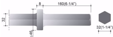
Shank: \varnothing 32x160mm
