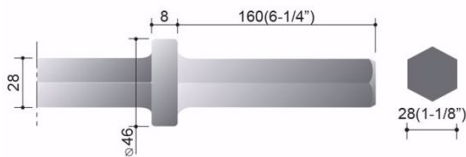
Shank: \varnothing 28 \times 160 mm
