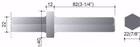
Shank: 22x82mm
