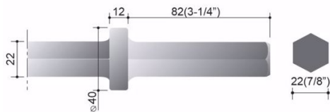
Shank: 22x82mm
