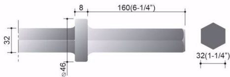
Shank: \varnothing 32 \times 160 mm
